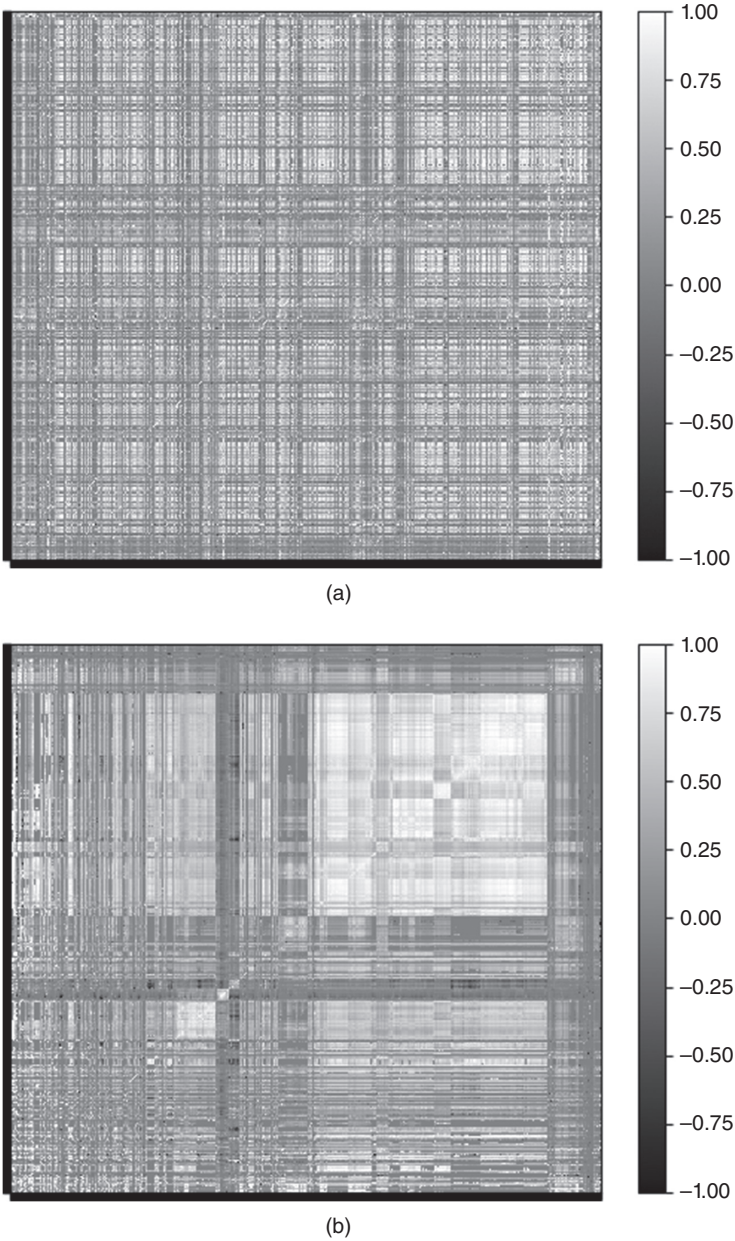
FIGURE 16.8 Correlation matrix before and after clustering The methodology described in this chapter can be applied to problems beyond optimization. For example, a PCA analysis of a large fixed income universe suffers the same drawbacks we described for CLA. Small-data techniques developed decades and centuries ago (factor models, regression analysis, econometrics) fail to recognize the hierarchical nature of financial big data.
